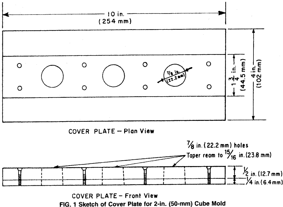
FIG. 1 Sketch of Cover Plate for 2-in. (50-mm) Cube Mold
